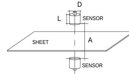
Fig. 3 Sensor / sheet arrangement Sensor dimensions: Page 12
