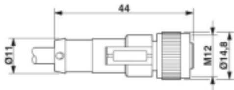
Fig. 4 Connector dimensions
