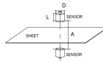
Fig. 4 Sensor / sheet arrangement Sensor dimensions: Page 12
