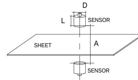
Fig. 4 Sensor / sheet arrangement Sensor dimensions: Page 12
